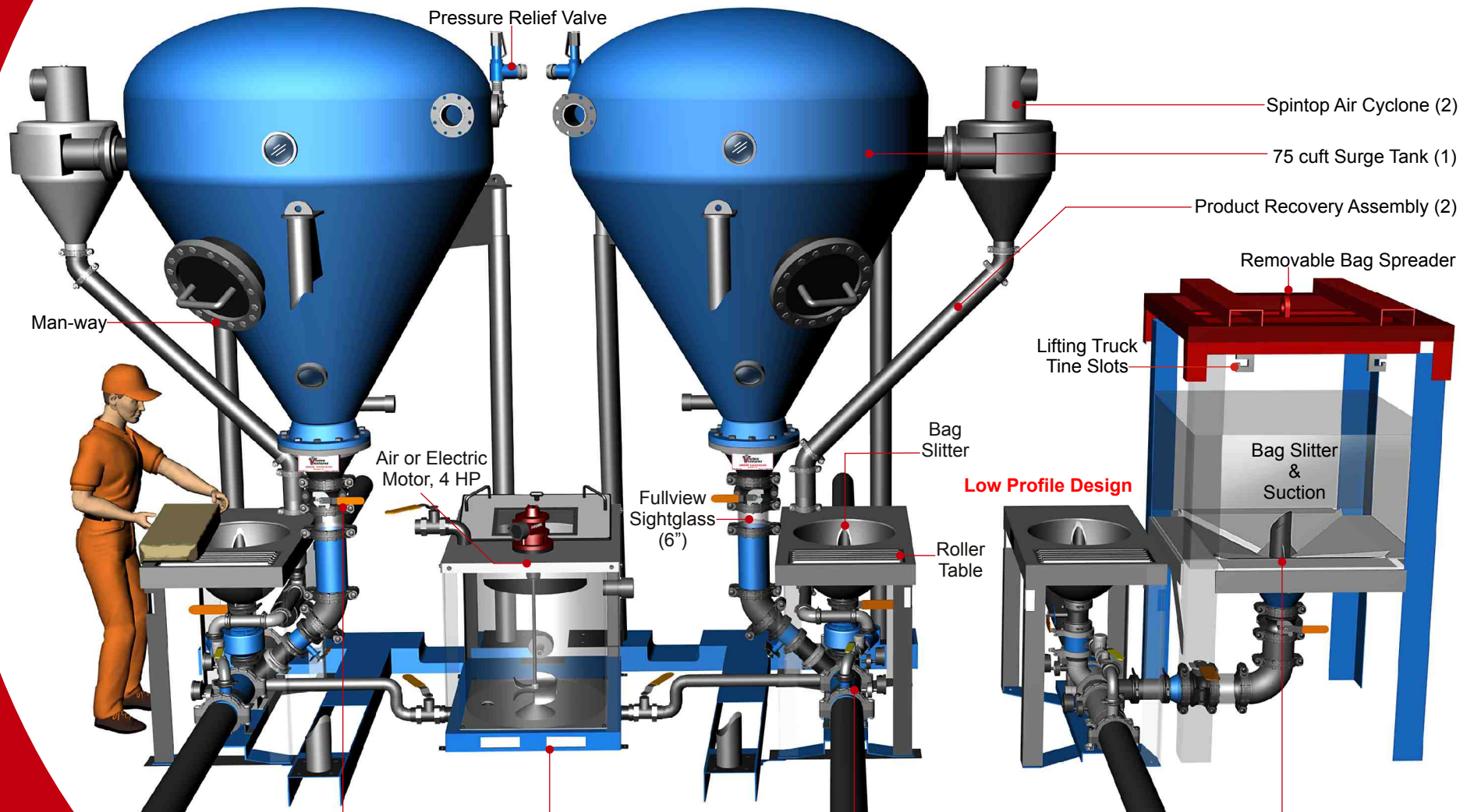
V-SLIDE ASSEMBLY™ Model V-VS-12-M1
